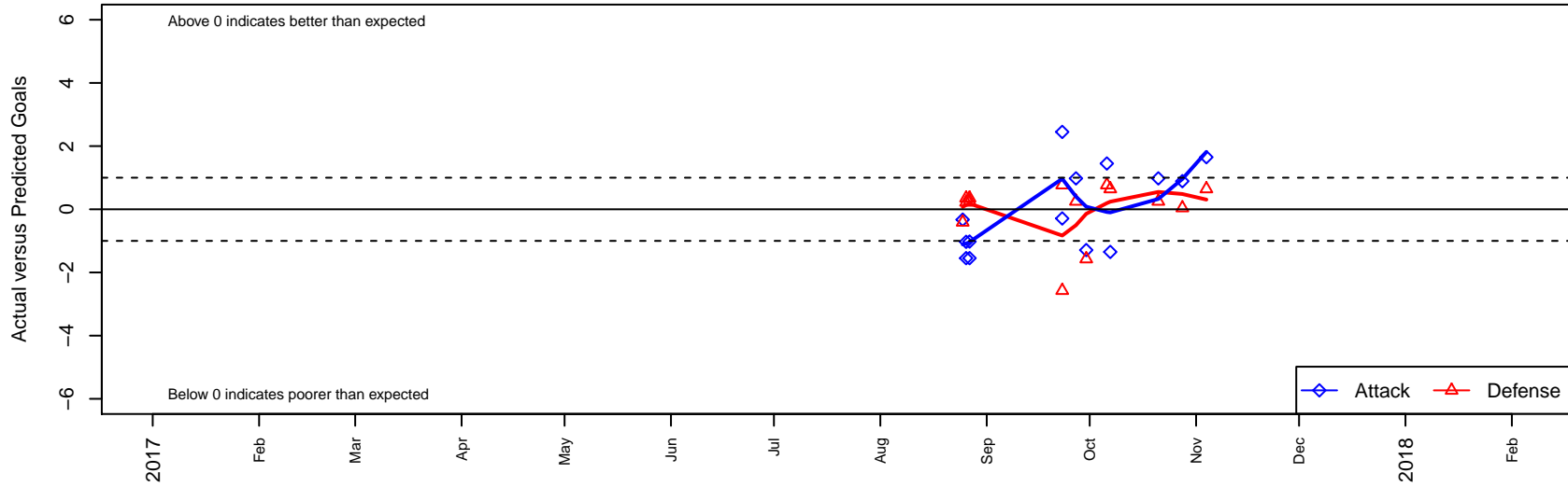
Spokane Foxes Chaos G05 Dots are actual minus expected GF (blue circles) and GA (red triangles). Blue line is smoothed change in attack strength. Red is smoothed change in defense strength.
